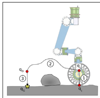
Figure 9. Execution of a step along a planned, obstacle-free path.
