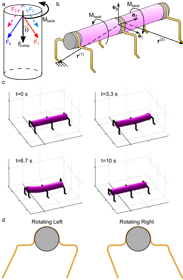
Fig. 4. (a) Model of cylindrical structure with forces from the actuators. (b) Model of a robot showing an example of how the axis of rotation is defined for both legs when the front, right and rear, left feet remain on the ground. This model also shows how the local coordinate frame, \mathbf{e}_i , is defined. (c) Example simulation demonstrating a robot walking with \theta = 26.5^\circ . (d) Diagram showing how to adjust the legs for rotating as seen by the front of the robot.
